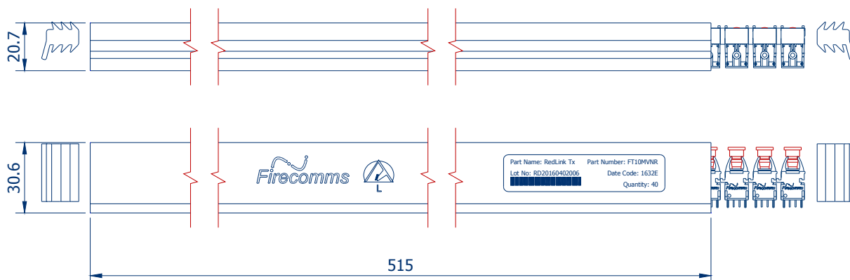
FIGURE 13 Packing tube for Firecomms Vertical RedLink® Transmitters
