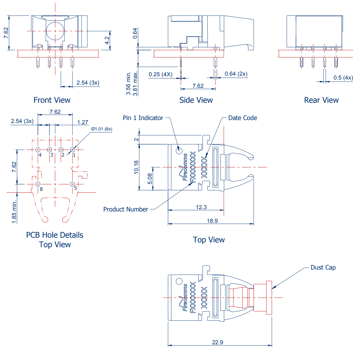
FIGURE 10 Mechanical dimensions of the horizontal connectors and PCB footprint, which is a top view General dimensional tolerance is \pm 0.2 mm
