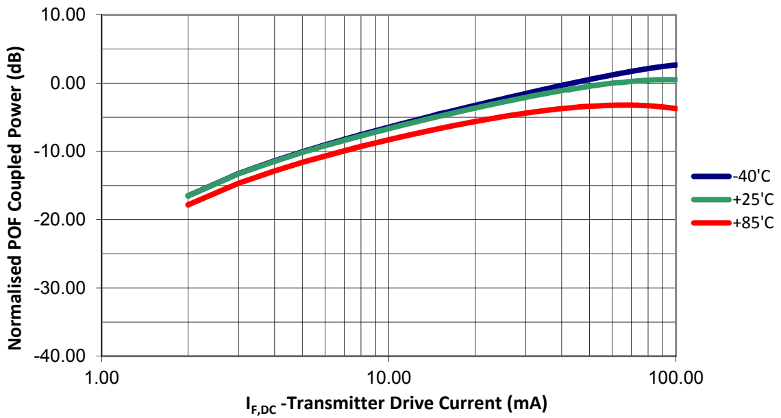
FIGURE 5 Typical normalized optical power vs. drive current.
