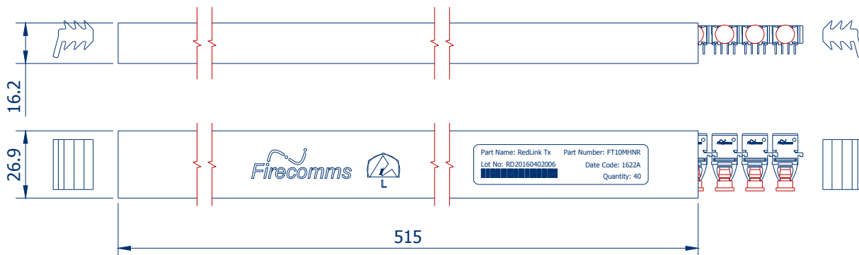
FIGURE 11 Packing tube for Firecomms Horizontal RedLink® Transmitters
