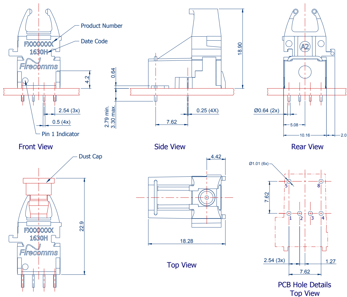
FIGURE 12 Mechanical dimensions of the vertical transmitter connectors and PCB footprint, which is a top view General dimensional tolerance is \pm 0.2 mm
